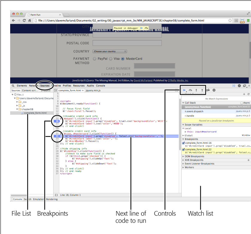
FIGURE 17-6 A debugger lets you set breakpoints (lines where the script stops and waits), control the execution of the script, and watch variables in the Watch list. As the debugger executes the script, the current line (the one that's about to run) is highlighted.
